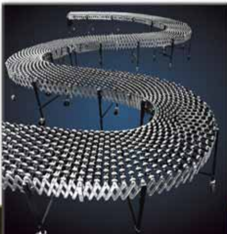
The original BEST/FLEX® flexible expandable conveyor.
