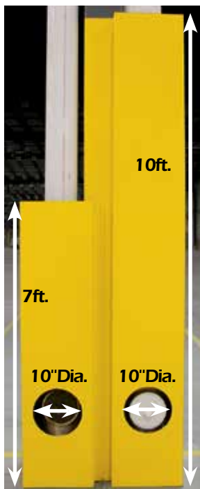
Downspout guards
